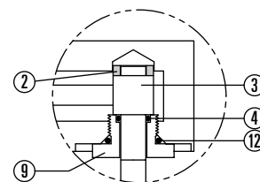
TRUNNION DETAIL
